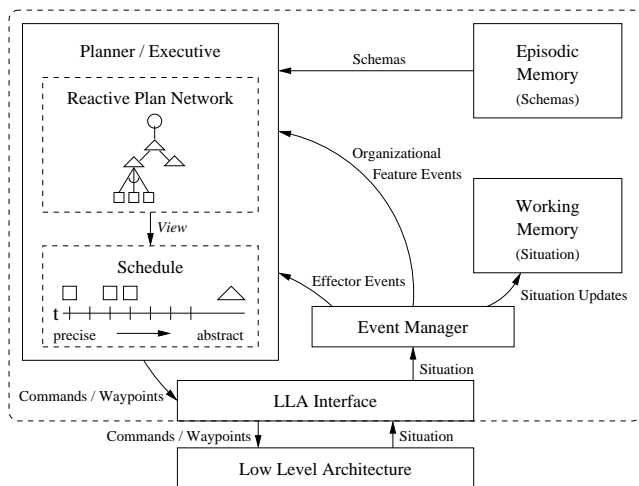
Figure 3: Orca's Knowledge Components
