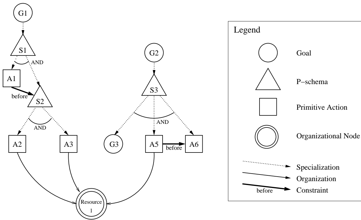
Figure 2: A Simple Reactive Plan Network
