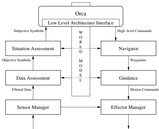
Figure 1: Orca situated in the MSEL software architecture
